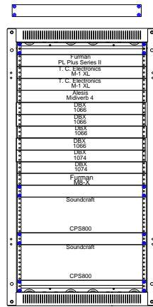
Middle Atlantic Products ERK-2125
